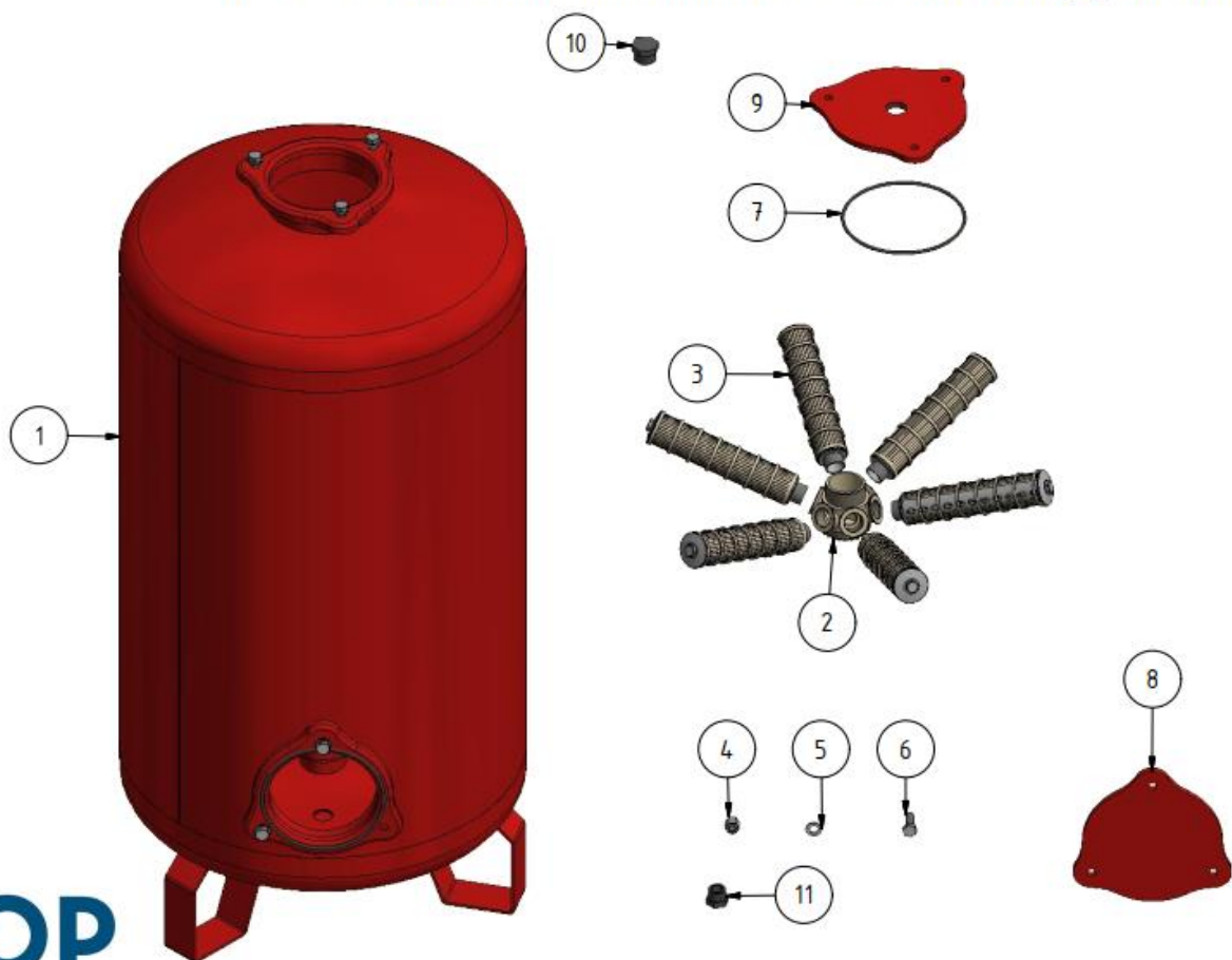
05-08-302 Sand media filter series 3"-24" without by-pass TF
