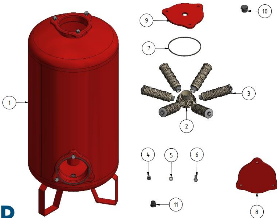
05-08-202 Sand media filter series X2"-20" without by-pass TF
