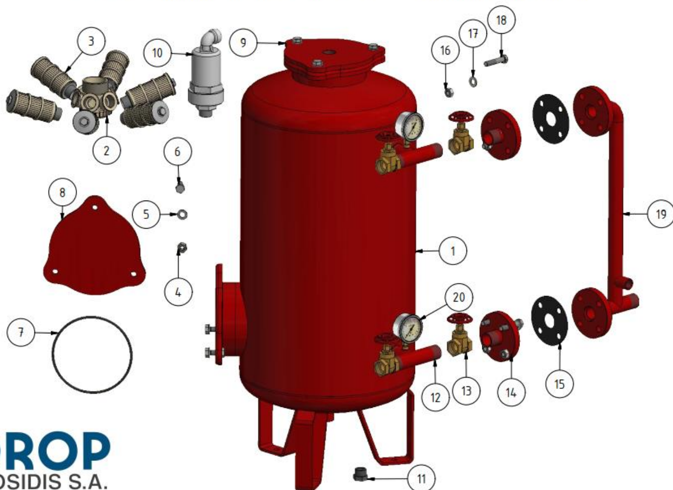
05-08-112 Sand media filter series X 1''-16'' manual with by-pass
