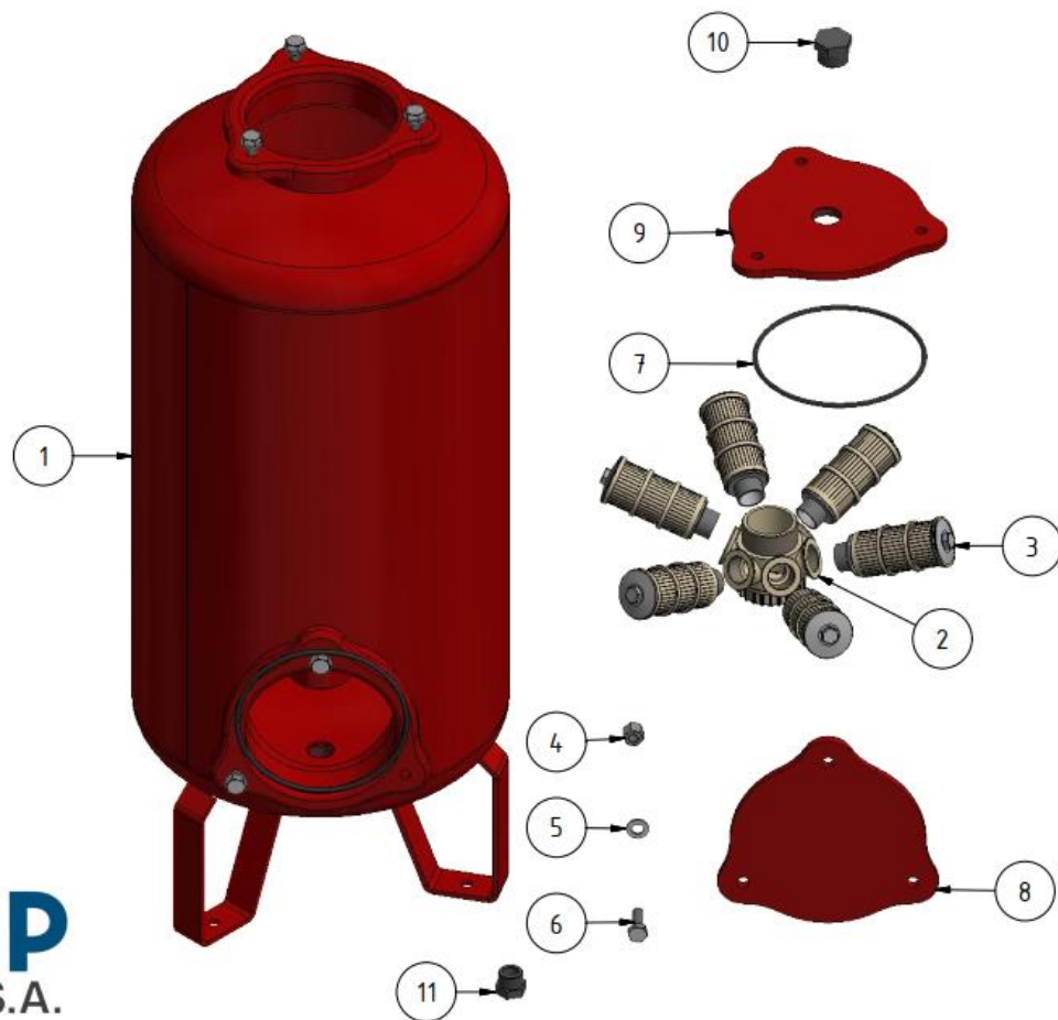
05-08-111 Sand media filtes series X 1''-16'' without by-pass TF
